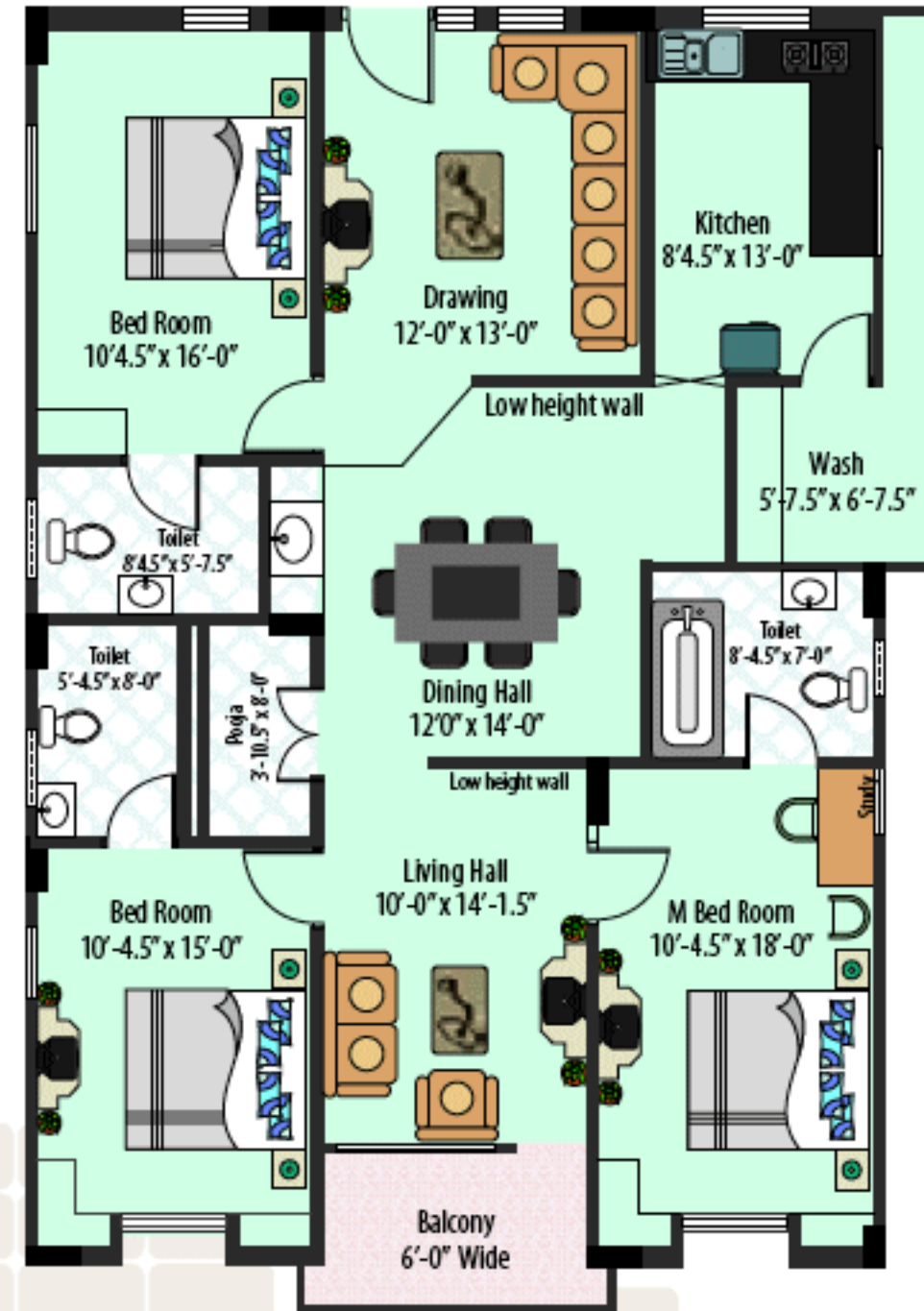
Block - 2, 3, 4, 6, 7 & 8 Area : 1905 Sft.
